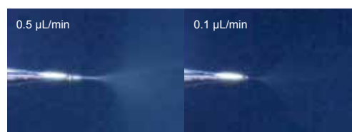
Change in Spray Shape at Different Flow Rates
